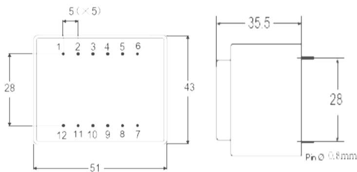
Dimension (mm)
